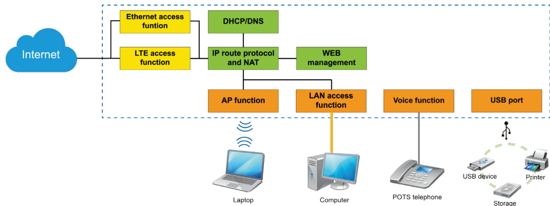
Figure 5-1 System architecture
